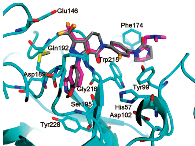
Figure 3. Superposition X-ray structures of fXa bound to compounds 40 and 4 . Atomic coloring is used with cyan for fXa cartoon and carbon atoms, gray for compound 40 carbon atoms, magenta for compound 4 carbon atoms, and orange for compound 4 fluorine atoms. The orientation is the same as in Figure 2. The figure was created using PyMol. 35
