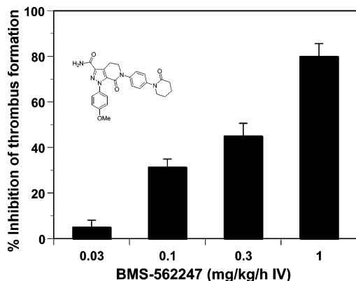
Figure 4. Rabbit arteriovenous shunt (AVShunt) profile of compound 40 (BMS-562247).
